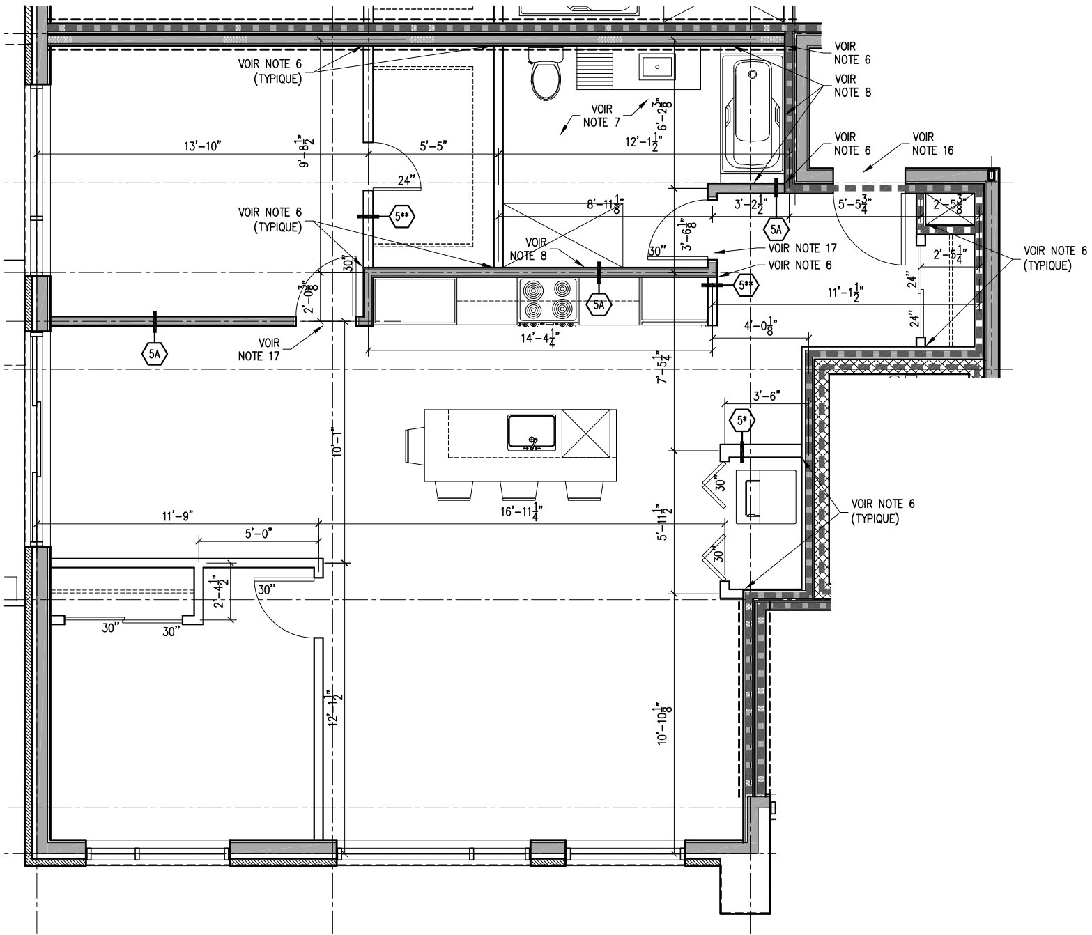
3 CONDO TYPE 6 (#101, #201, #301) A-107 ÉCHELLE: 1/4" = 1'-0"
