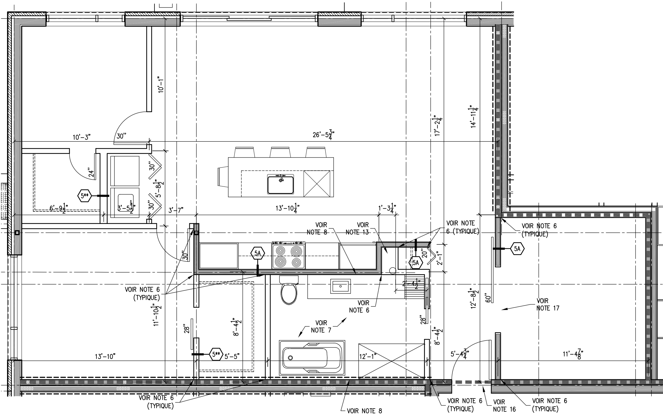
4 CONDO TYPE 5 (#102) A-107 ÉCHELLE: 1/4" = 1'-0"
