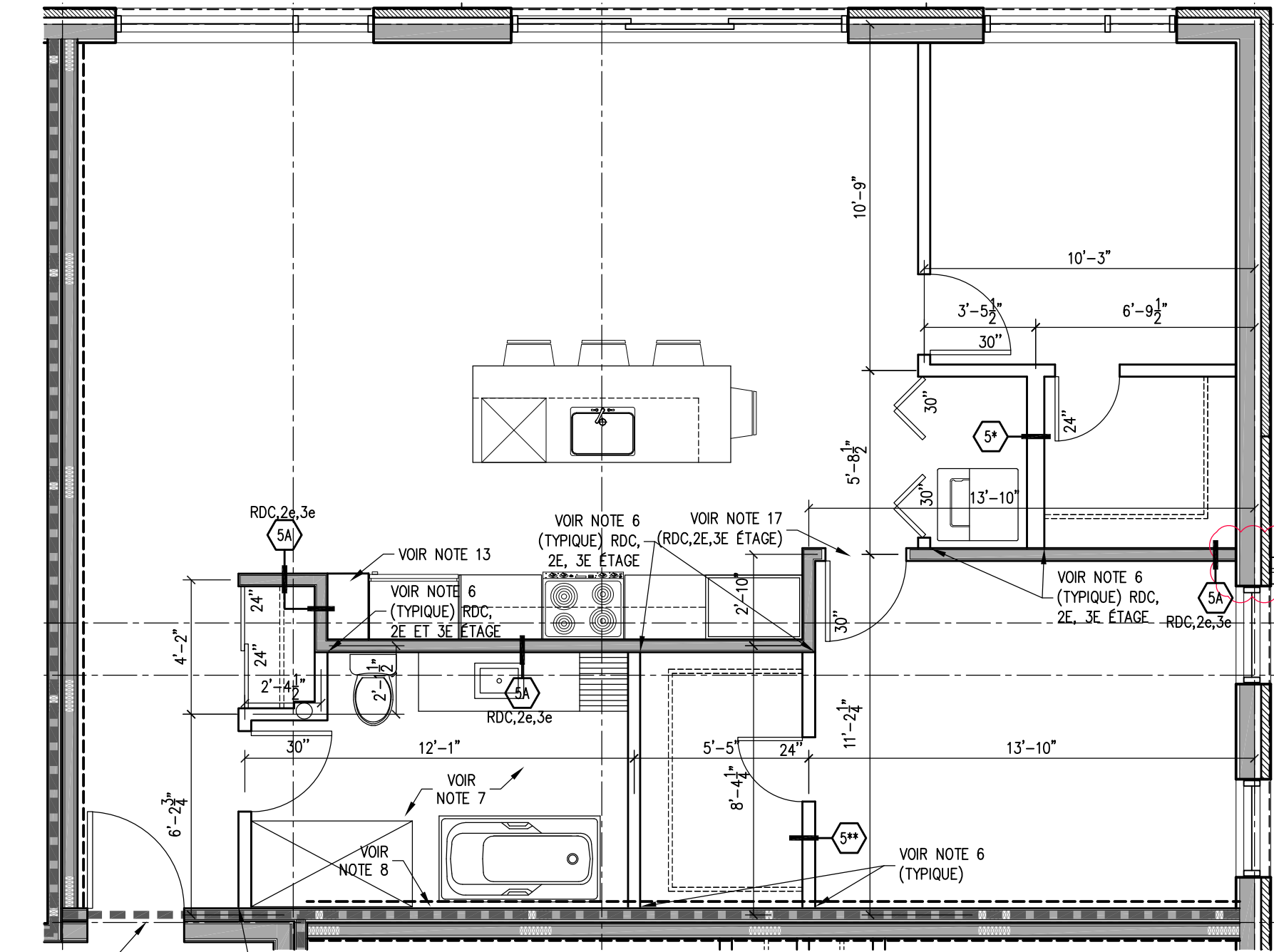
4 CONDO TYPE 3 (#104, #205, #305, #405) A-106 ÉCHELLE: 1/4" = 1'-0"
