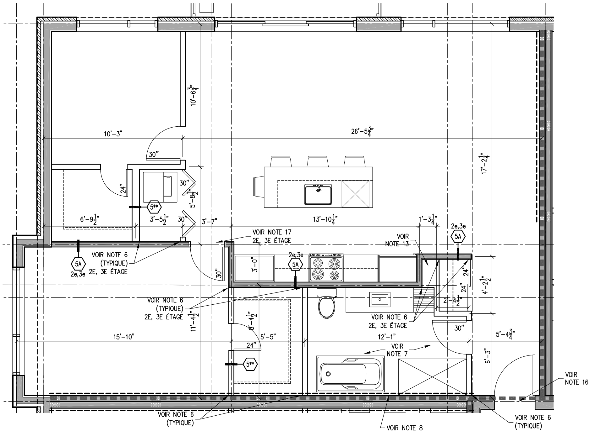
2 CONDO TYPE 5A (#202, #302, #402) A-107 ÉCHELLE: 1/4" = 1'-0"
