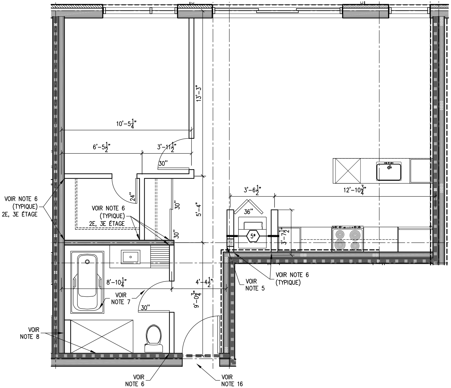
2 CONDO TYPE 8 (#204, #304, #404) A-108 ÉCHELLE: 1/4" = 1'-0"
