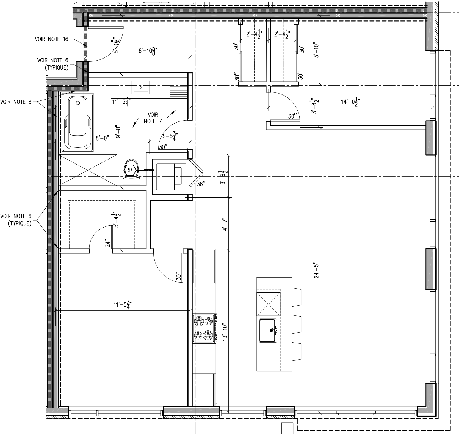
4 CONDO TYPE 2A (#406) A-108 ÉCHELLE: 1/4" = 1'-0"
